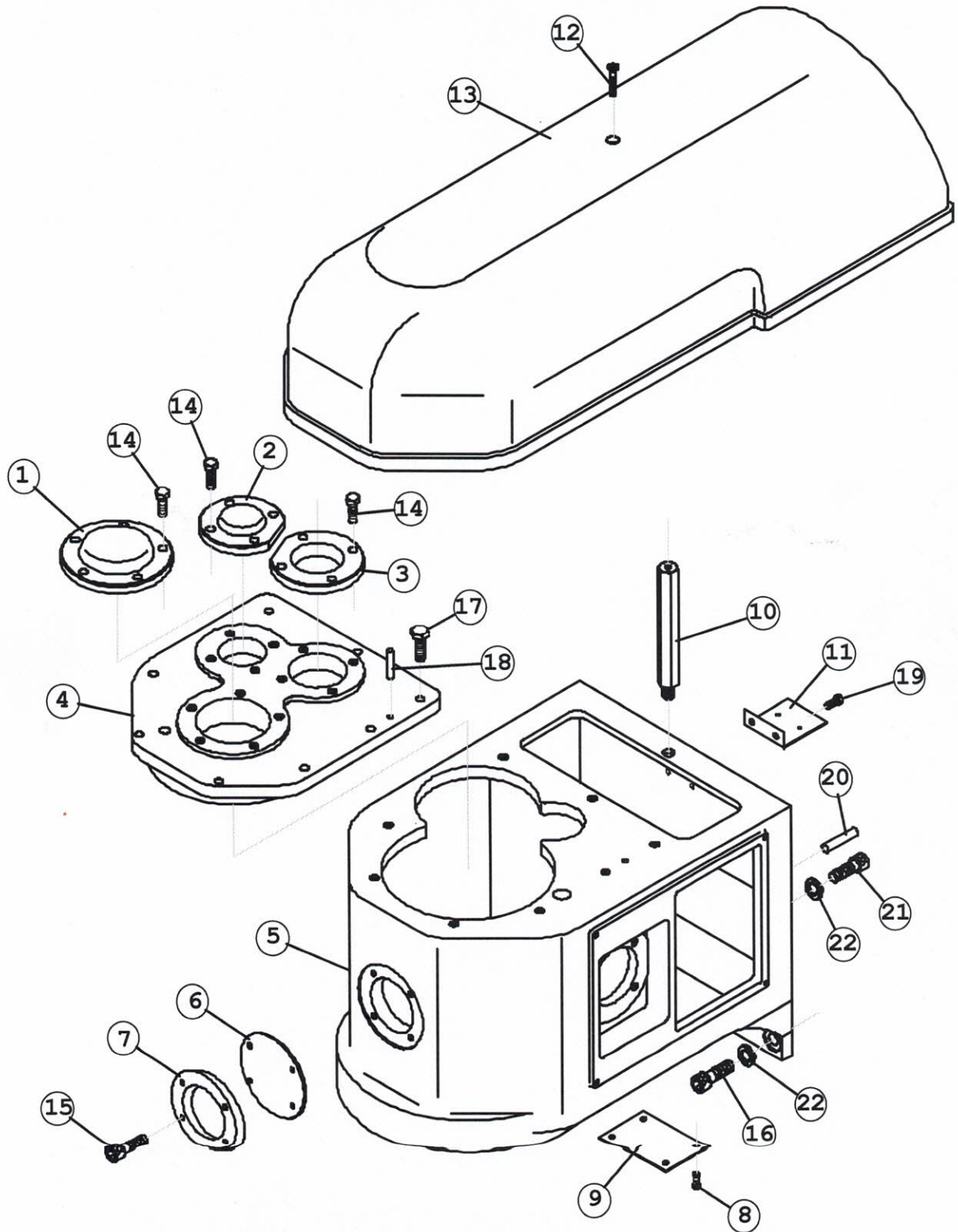
Figure 1. TRANSMISSION CASE
