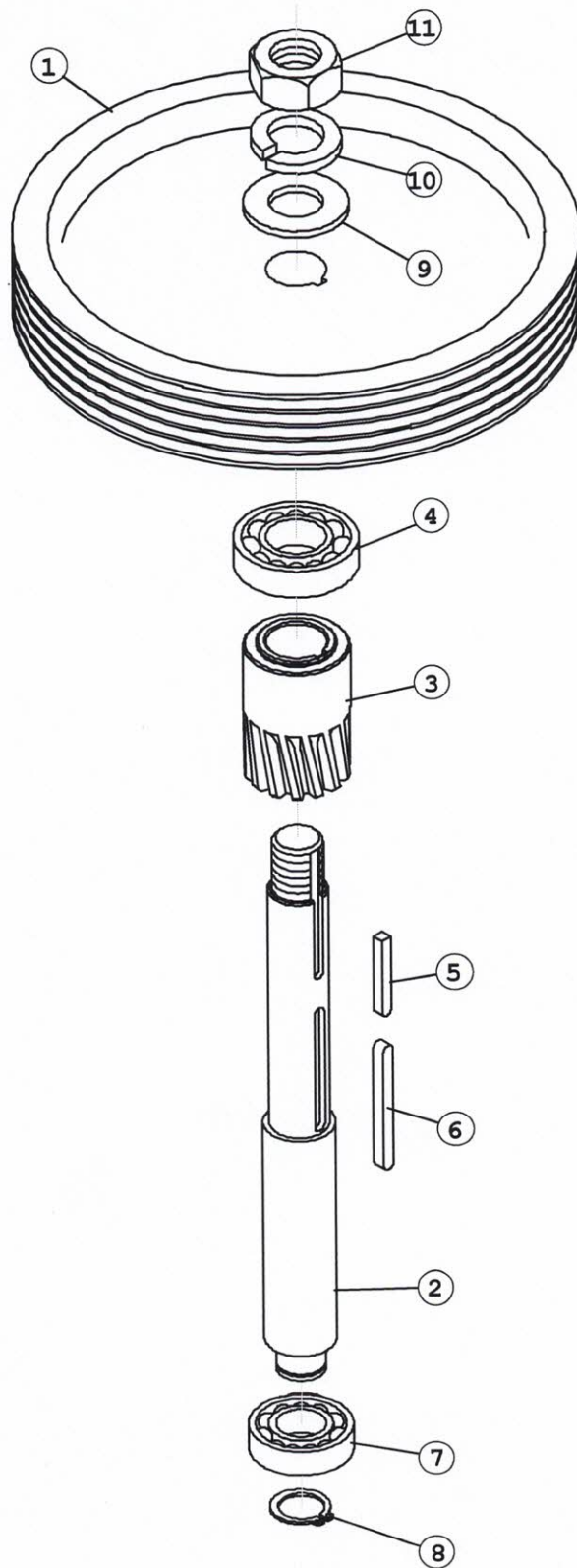
Figure 3. TRANSMISSION SHAFT
