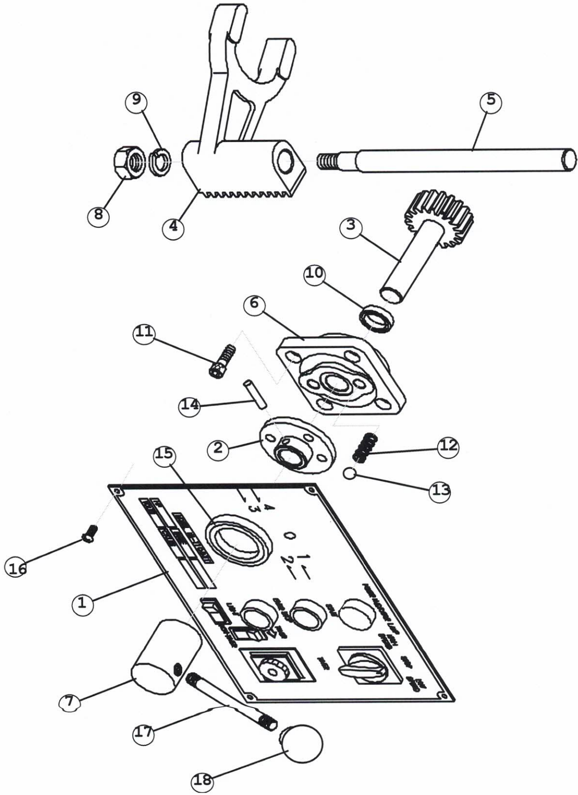
Figure 7. SHIFTER UNIT
