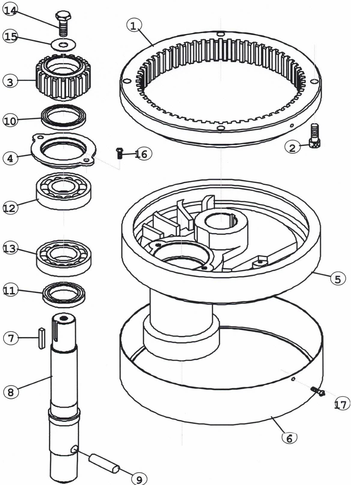
Figure 8. PLANETARY HEAD
