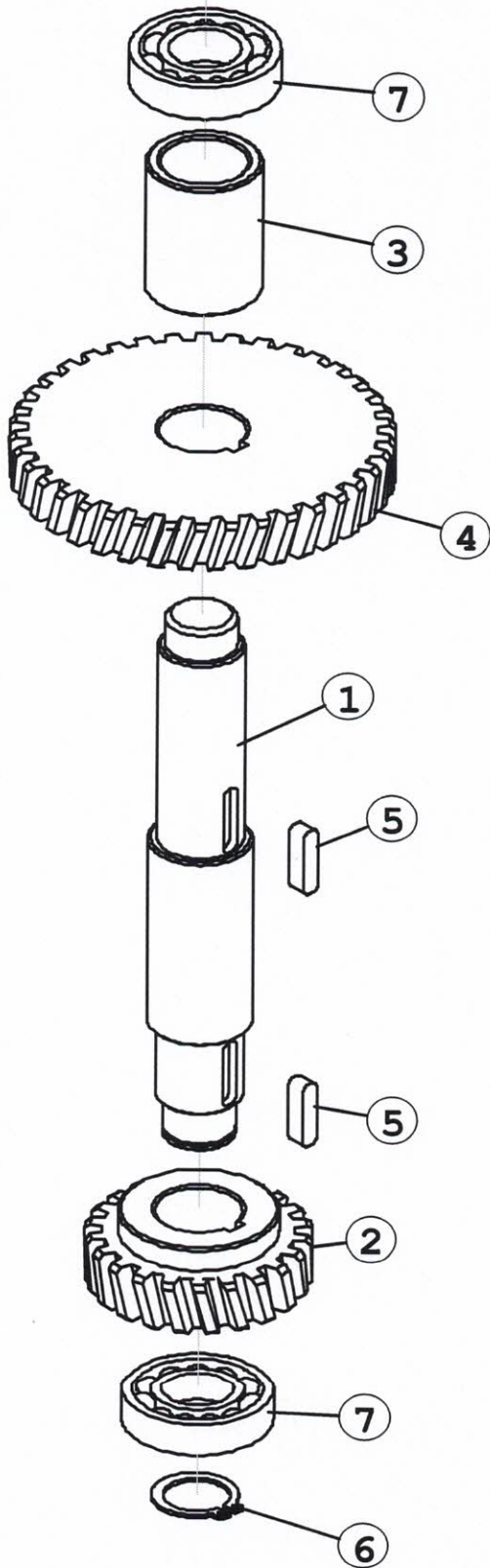
Figure 4. REDUCTION GEAR SHAFT
