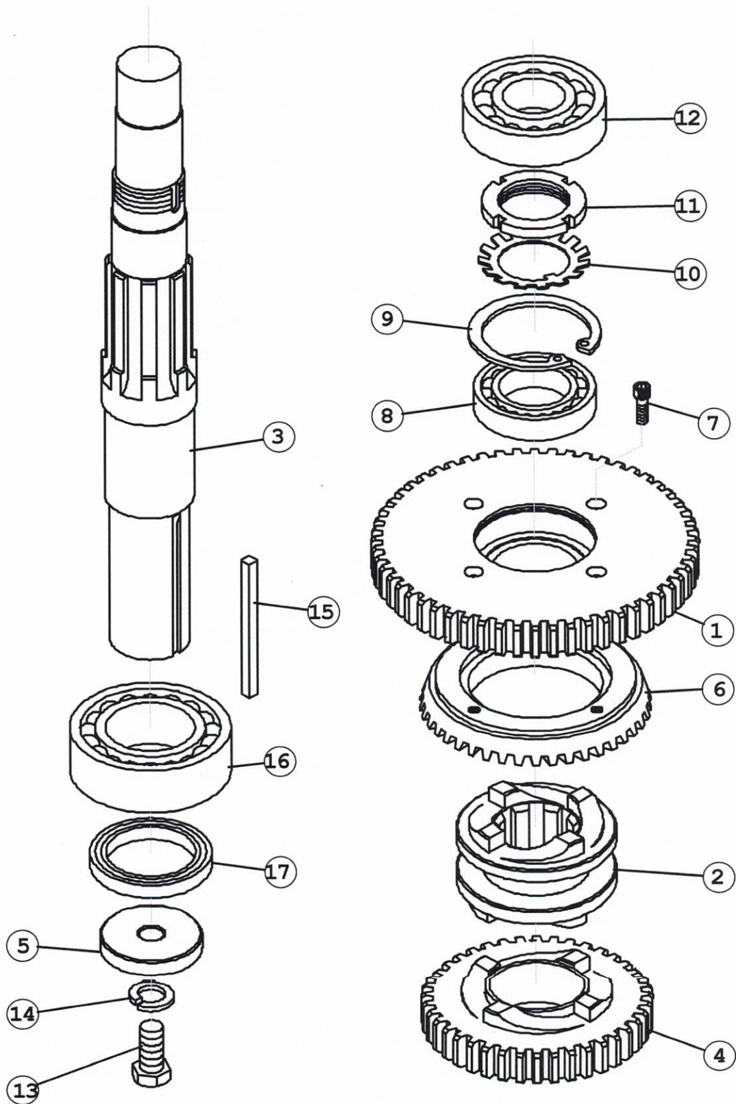
Figure 2. PLANETARY SHAFT
