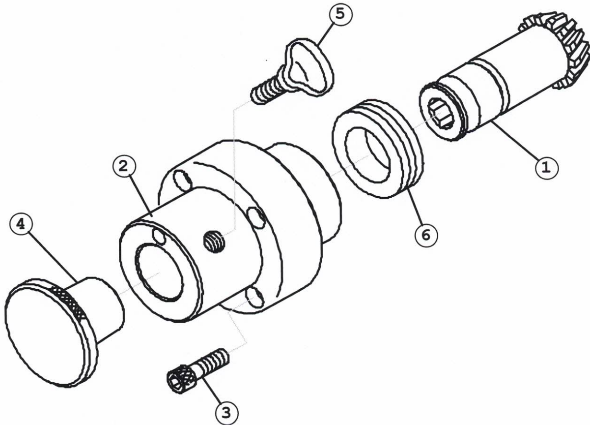
Figure 6. HUB ATTACHMENT
