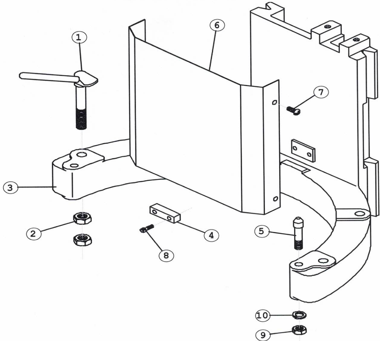
Figure 10. BOWL SUPPORT UNIT
